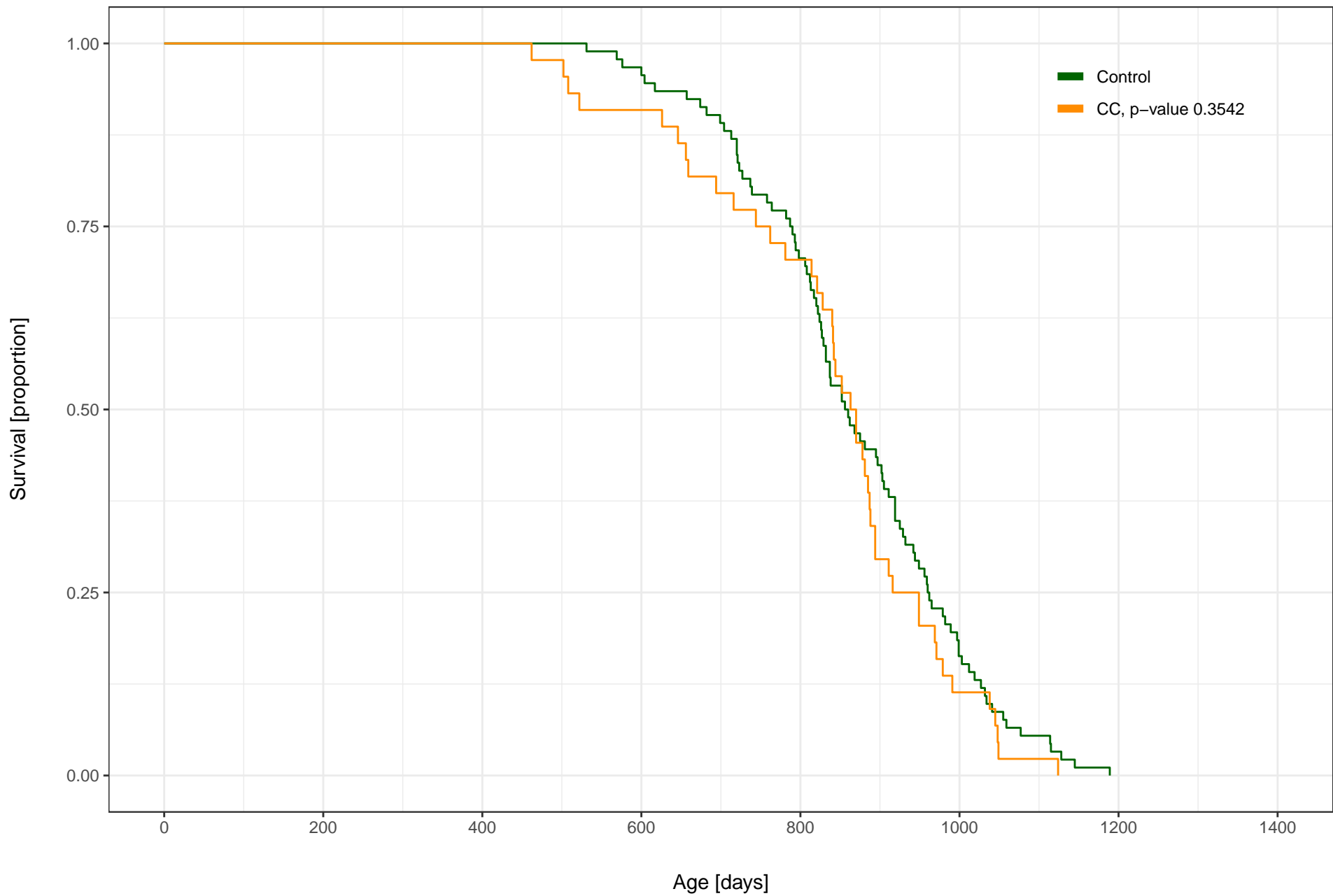
Cadesartan Cilixetil (30 ppm) vs. Control, Female, C2016 UM
