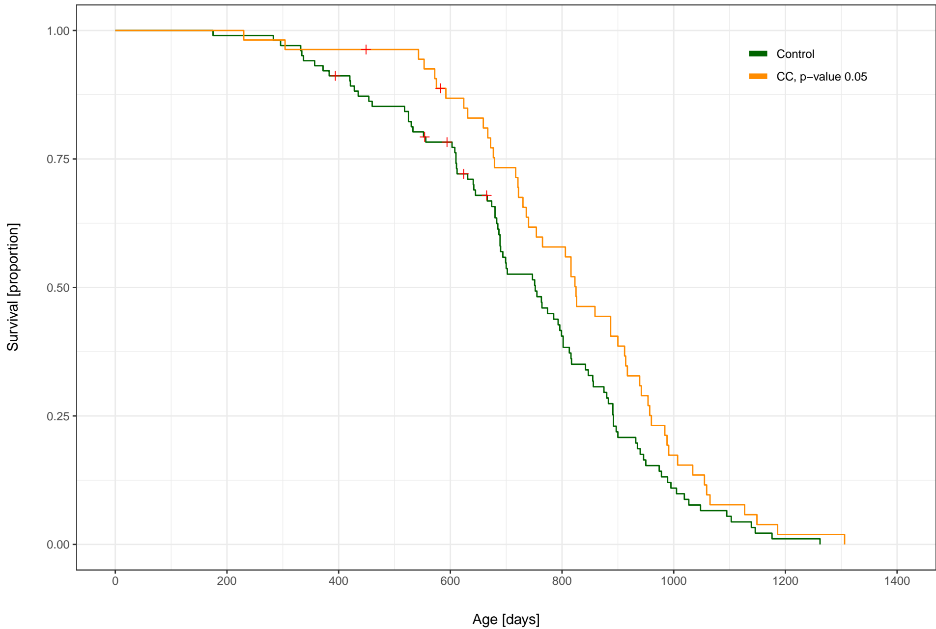
Cadesartan Cilexetil (30 ppm) vs. Control, Male, C2016 TJL
