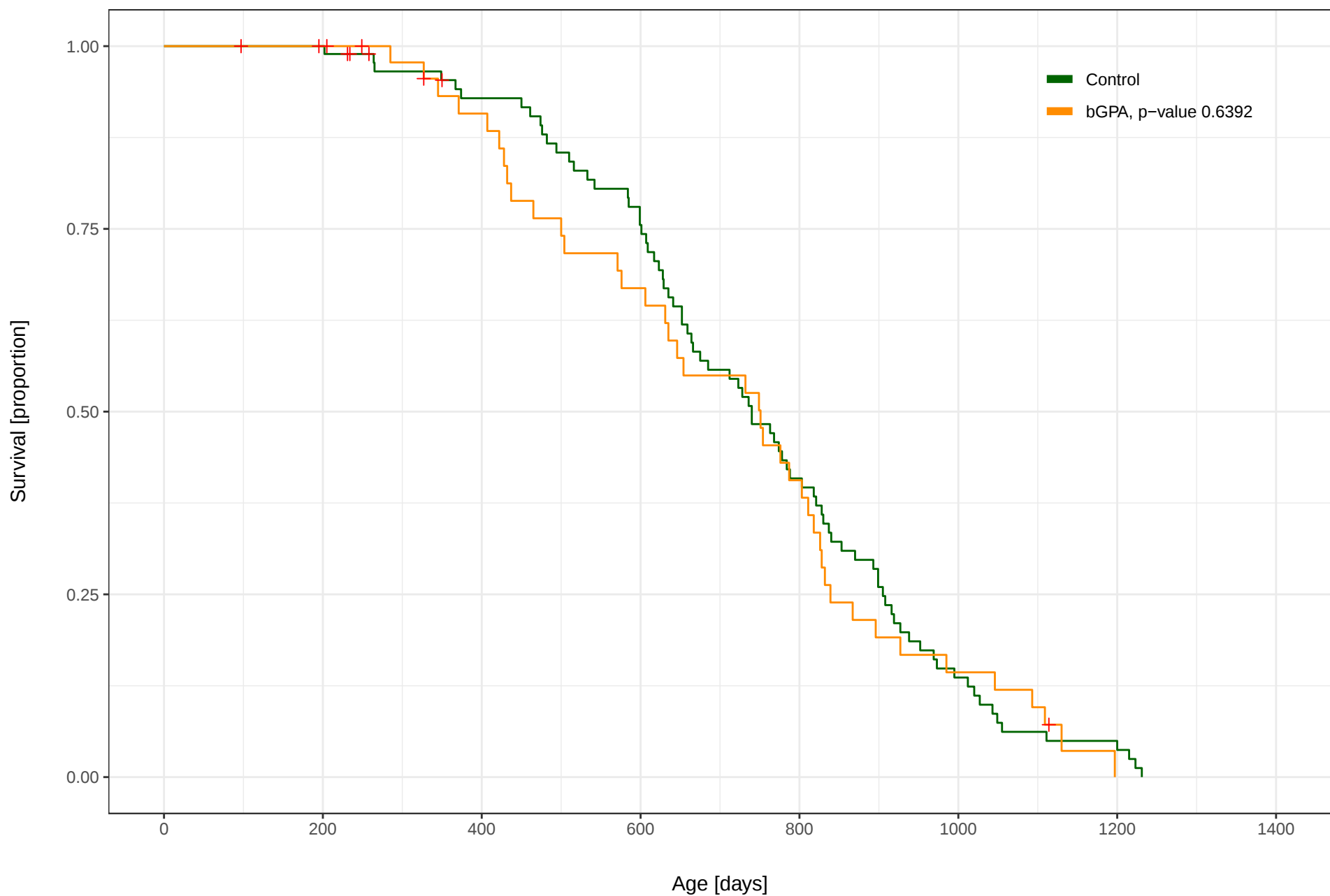
b-guanadinopropionic acid (3300 ppm) vs. Control, Male, C2015 UM
