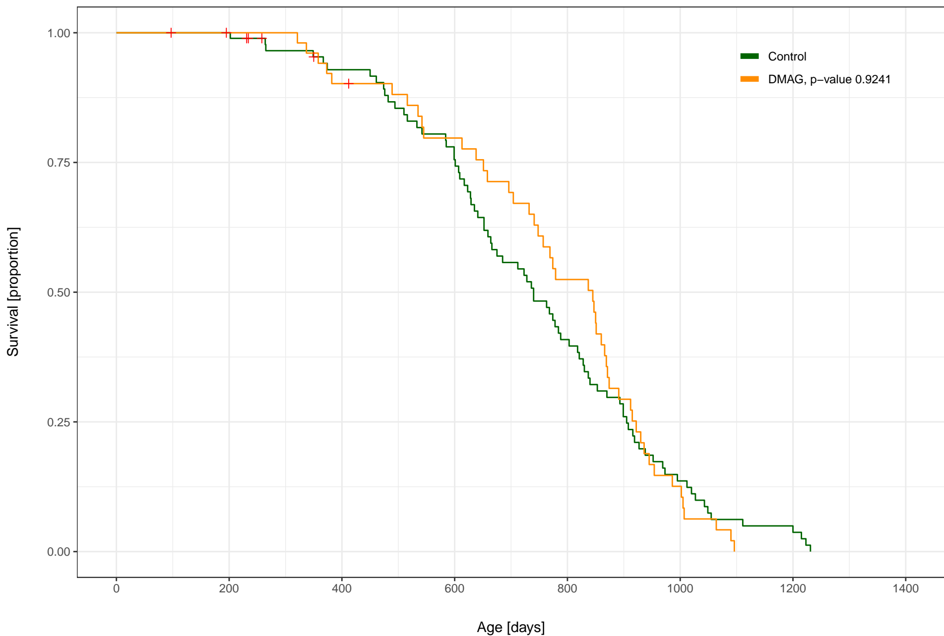
17-dimethylaminoethylamino-17-demethoxygeldanamycin hydrochloride (30 ppm) vs. Control, Male, C2015 UM
