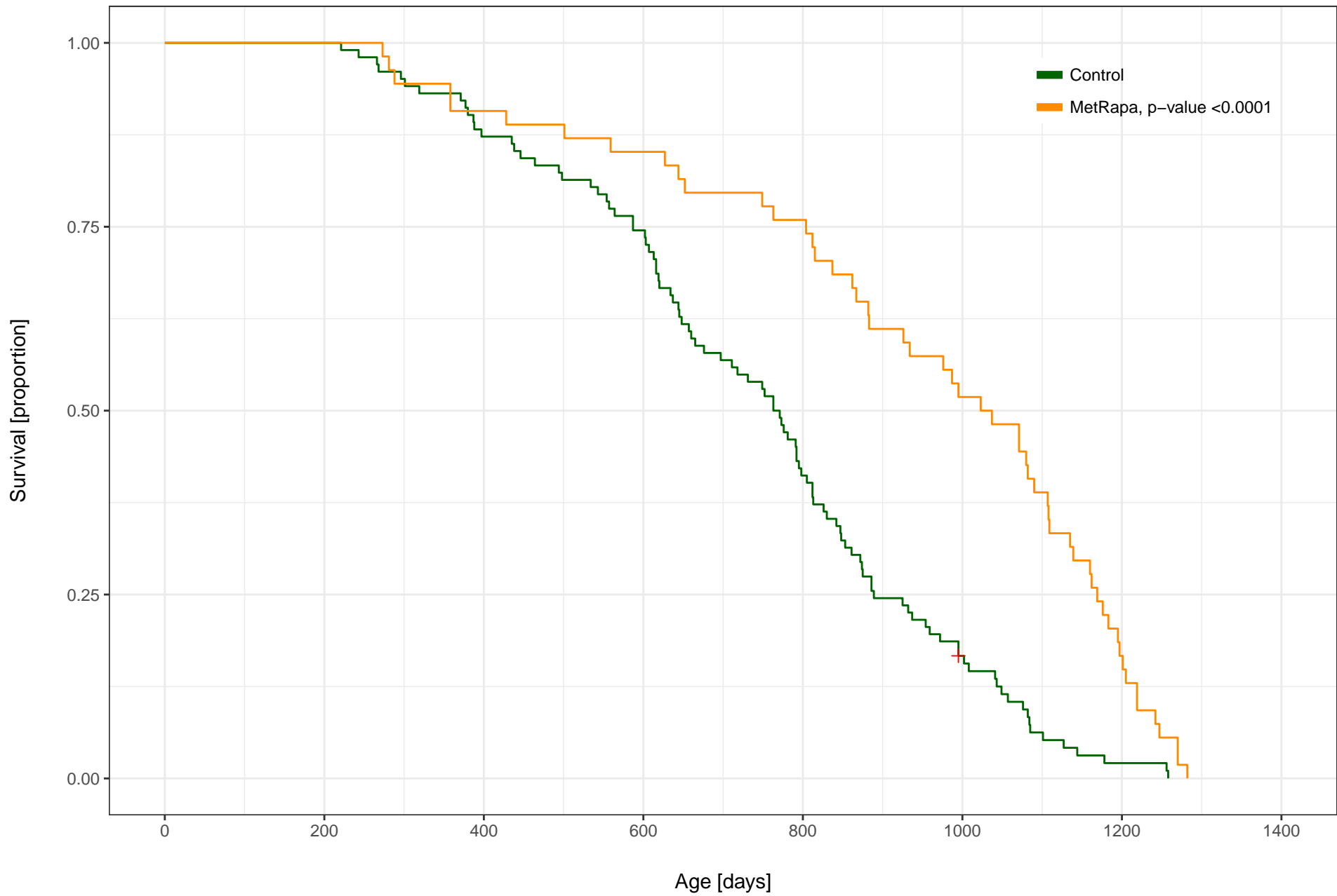
MetRapa (1000, 14 ppm) vs. Control, Male, C2011 TJL
