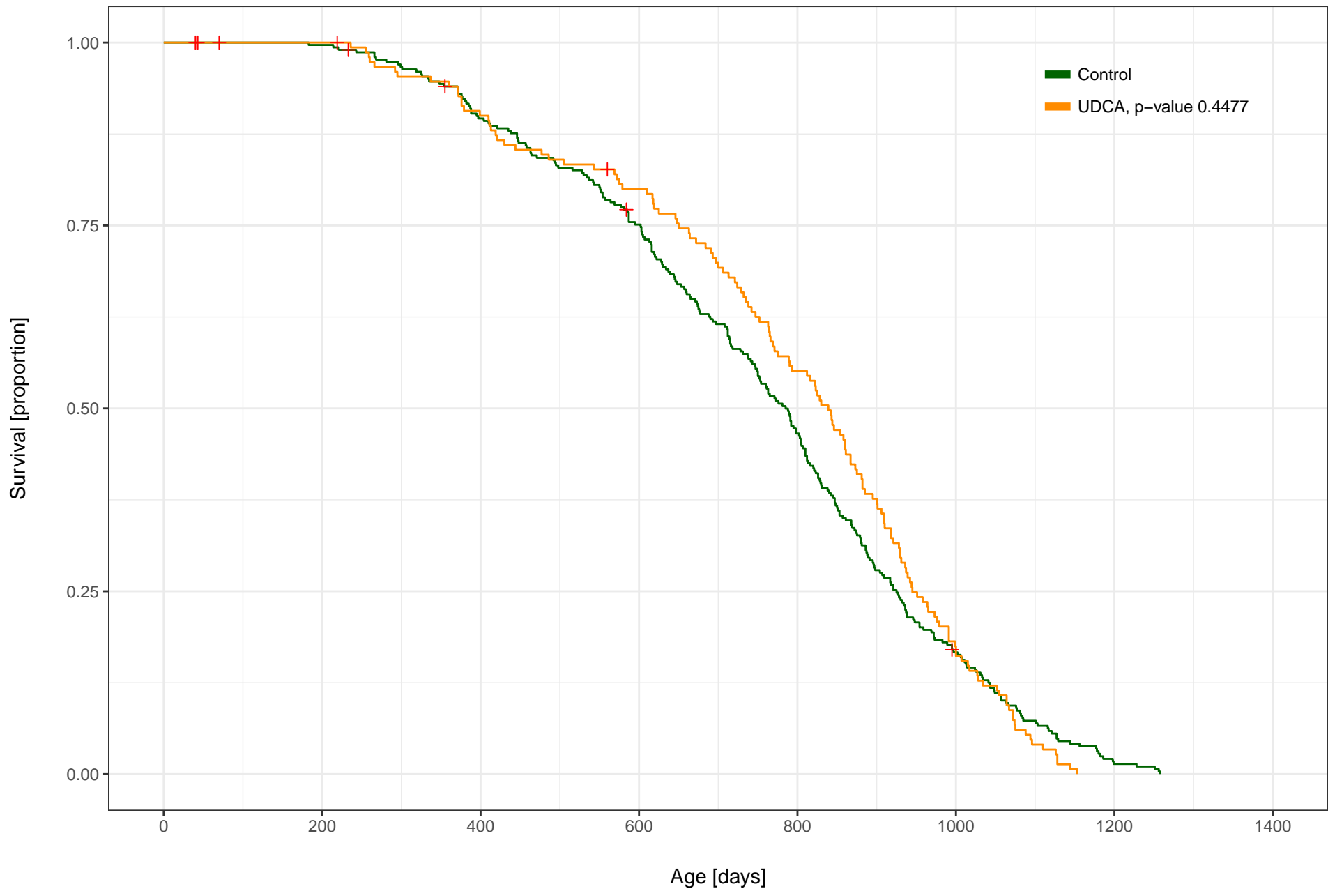
UDCA (5000 ppm) vs. Control, Male, C2011 All Sites
