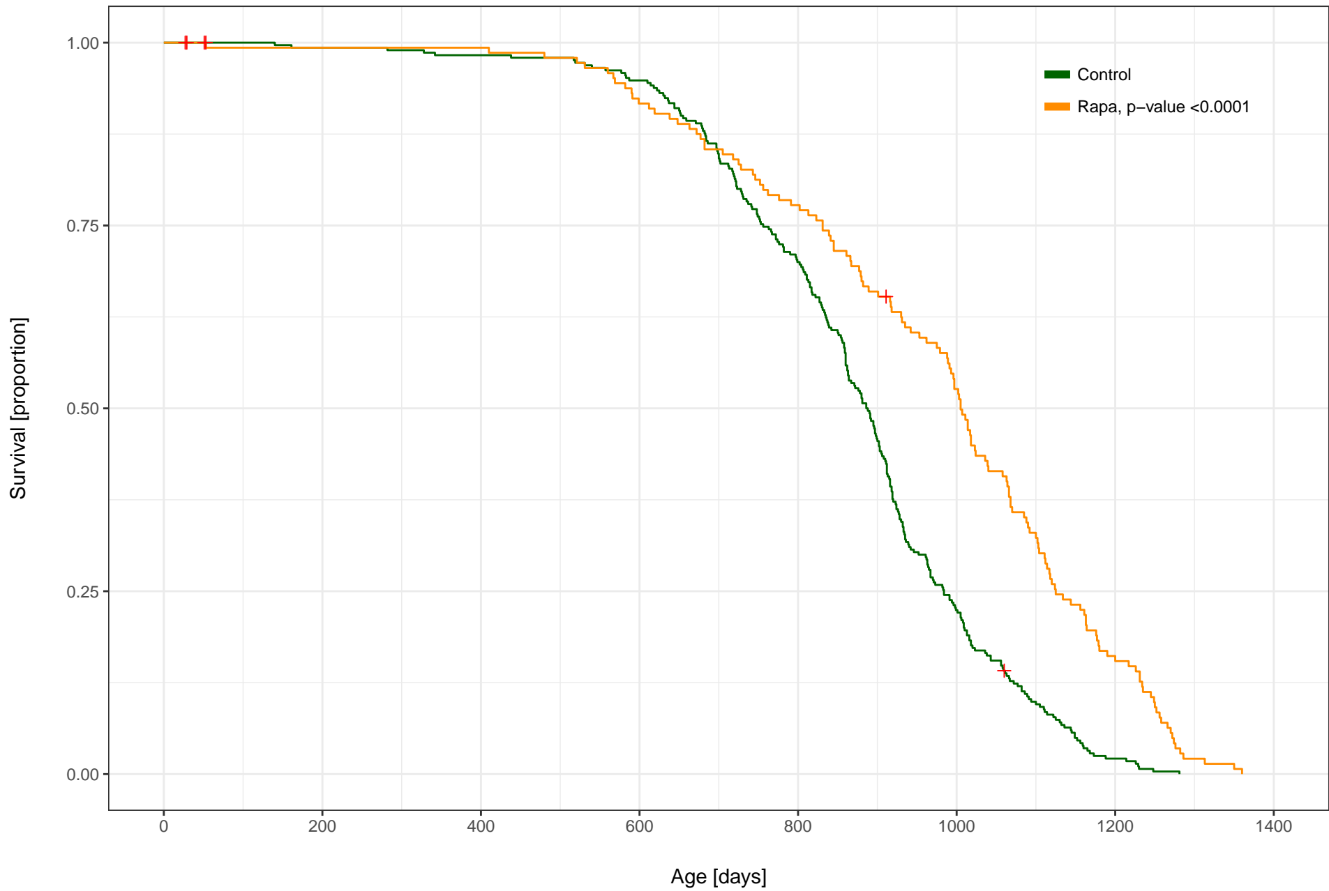
Rapa (14 ppm) vs. Control, Female, C2005 All Sites
