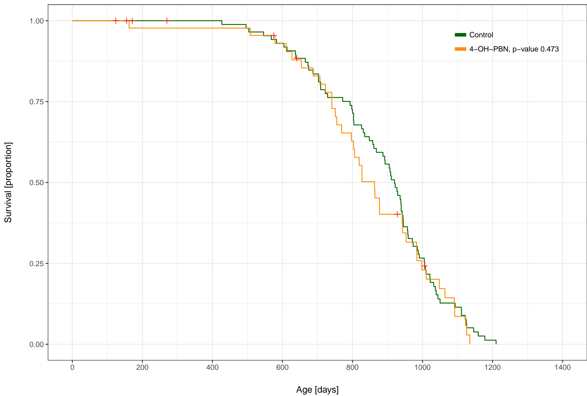
4-OH-PBN (315 ppm) vs. Control, Female, C2004 UM
