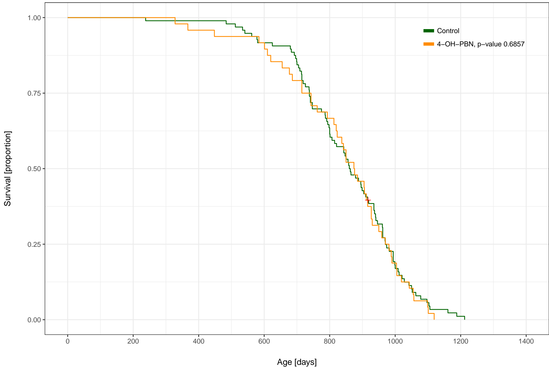
4-OH-PBN (315 ppm) vs. Control, Female, C2004 TJL
